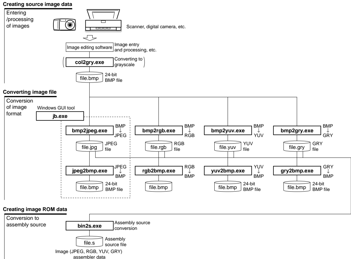
Figure 4.1.1 Flow Chart for Creating Image ROM Data
